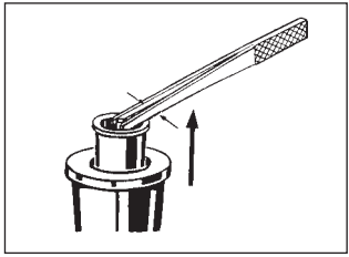
Fig. 1: Three-way switch in the engineer's cab Fig. 2: Pulling out the smoke generator insert. Fig. 3: Changing the smoke generator 1) Remove the old smoke generator. 2) Cut the wires. 3) Connect the new smoke generator. 4) Insulate the wires before inserting the new smoke generator.
